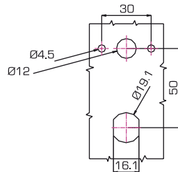
Panel Drilling
