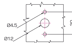
Panel Drilling
