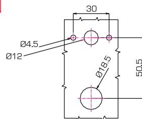
Panel Drilling
